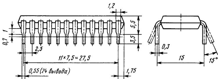
2120.24-1
