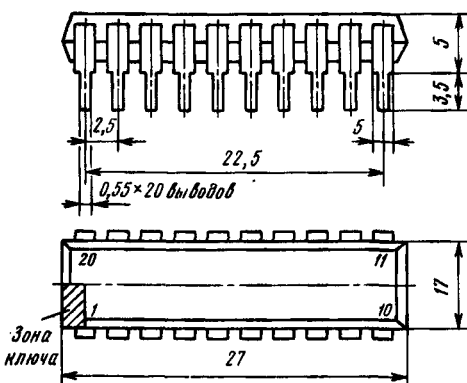
2140.20-1
