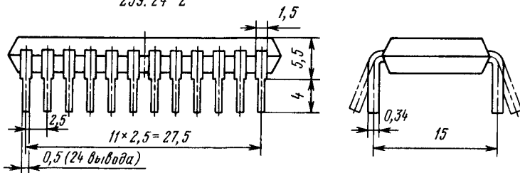
239.24-2
