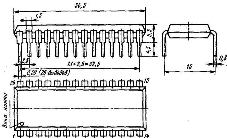
2121.28-12
