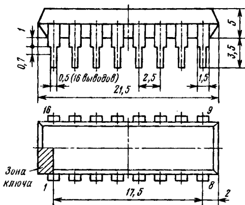
238.16-2
