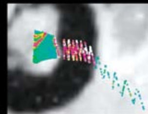
24INLOKIRA01 11 October 1999 UT 04:20 4.7 microns 1.3-2.1 km/pixel
